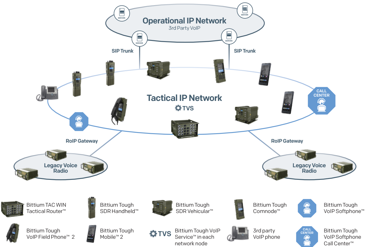
Figure 3: Trunk connections and legacy voice radio connectivity
